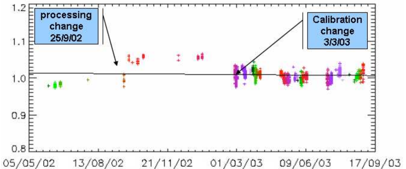
Figure 4. Temporal change in the MERIS calibration coefficient at 490 nm.
